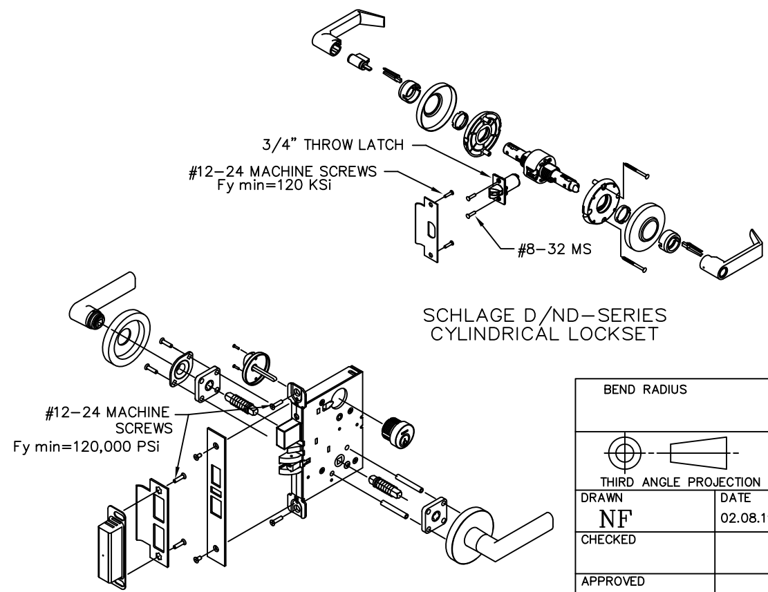
SCHLAGE L9400 SERIES MORTISE LOCKSET W/ DEADBOLT
