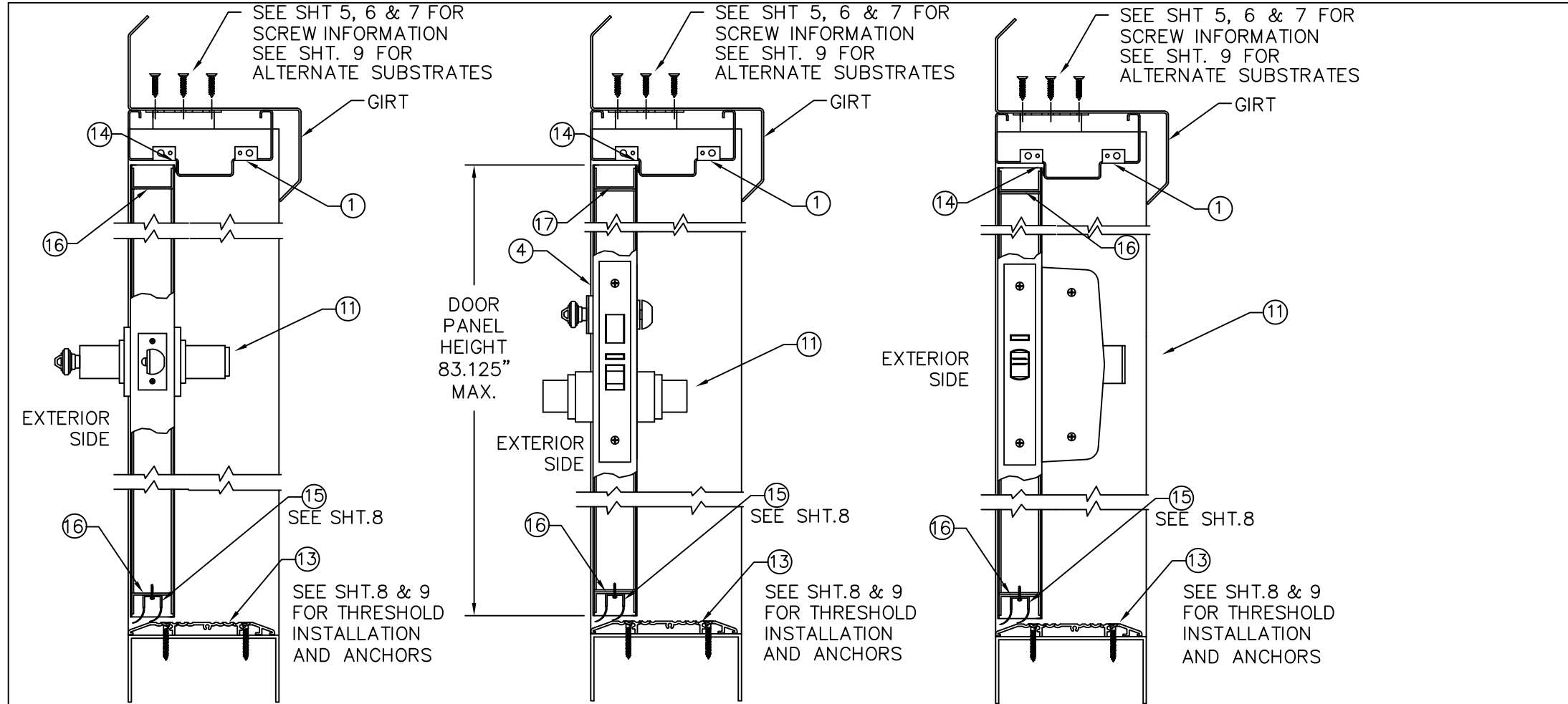
SECTION B-B CYLINDRICAL LOCKSET SCHLAGE D/ND-SERIES
