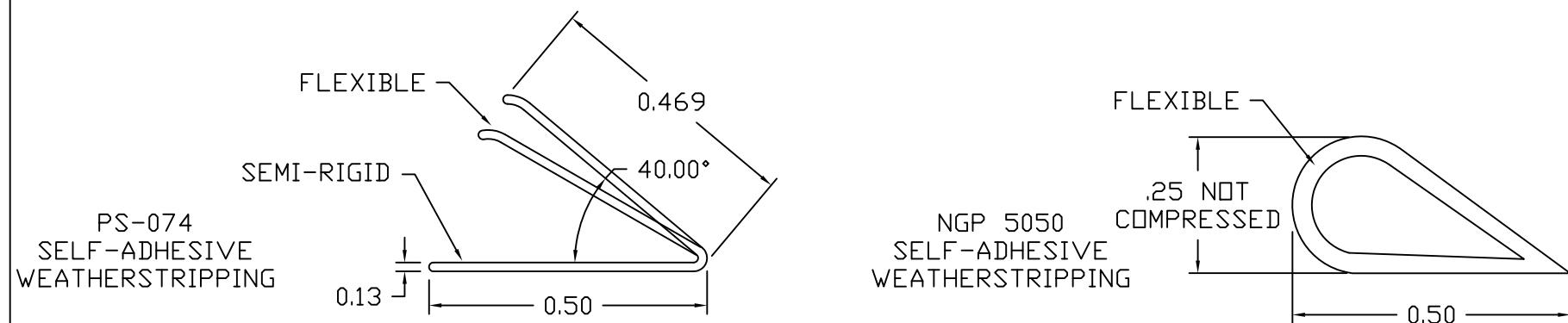
DETAIL A THRESHOLD PROFILE
