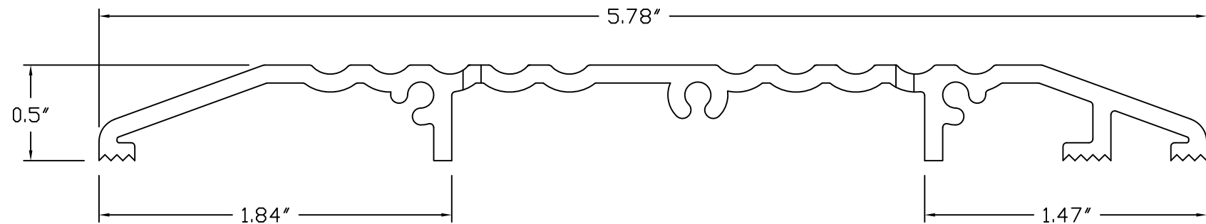
DETAIL A THRESHOLD PROFILE
